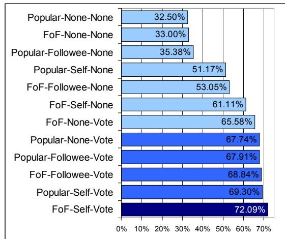
Figure 4. Percentage of Interesting URLs Recommended per Algorithm. FoF-Self-Vote at the bottom is significantly better than the top 7 algorithms in the list
