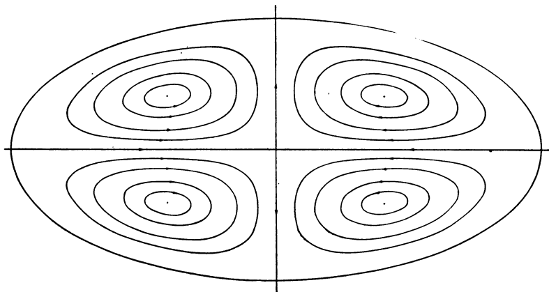
FIG. 1. Secondary flow in a tube with elliptical cross-section ( \alpha > 0 ).
