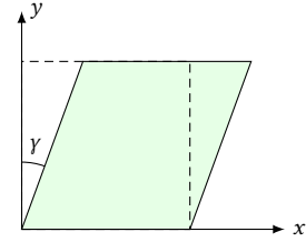
Figure 1.4: The tensor F maps the square (drawn in dashed lines) to the parallelogram (filled in light green). The square's vertical edge gets tilted by angle \gamma relative to the vertical.
