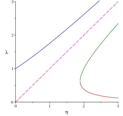
Figure 14.5: The solid lines depict the three roots of the equation (\eta - \lambda)^2 \lambda - 1 = 0 plotted against \eta . The roots plotted in red and green lie below the line \lambda = \eta , plotted in dashed magenta. The root plotted in blue lies above that line and is not of interest in the context of our application. The leftmost point of the red and green graphs is at \eta = \eta_{\text{cr}} \approx 1.89 .
