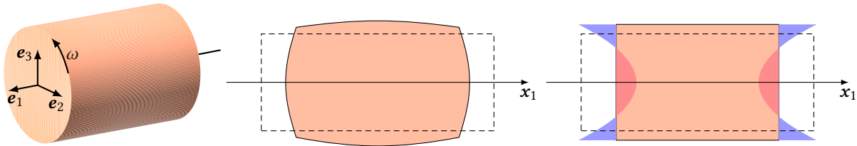
Figure 14.1: At the left, the rubber cylinder spinning about the \mathbf{e}_1 axis with angular velocity \omega . At the center, the dotted rectangle is the silhouette of the undeformed cylinder, while the filled region depicts the barreled shape of the spinning body when no surface tractions are applied. At the right, self-equilibrated tractions, indicated by their distribution profiles, applied to the spinning cylinder's bases, force it into a cylindrical shape.
