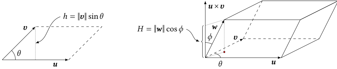
Figure 1.1: On the left: The area A of the parallelogram formed by the vectors \mathbf{u} and \mathbf{v} is A = \|\mathbf{u}\| h = \|\mathbf{u}\| \|\mathbf{v}\| \sin \theta = \|\mathbf{u} \times \mathbf{v}\| . On the right: The (signed) volume V of the parallelepiped formed by the vectors \mathbf{u}, \mathbf{v}, \mathbf{w} is the area of the base times the height, that is V = \|\mathbf{u} \times \mathbf{v}\| H = \|\mathbf{u} \times \mathbf{v}\| \|\mathbf{w}\| \cos \phi = (\mathbf{u} \times \mathbf{v}) \cdot \mathbf{w} = [\mathbf{u}, \mathbf{v}, \mathbf{w}] .
