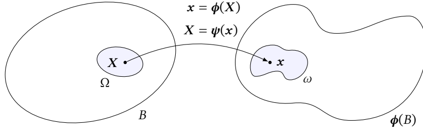
Figure 7.1: The deformation \phi maps the body B \subset \mathcal{E}_3 to \phi(B) \subset \mathcal{E}_3 . The inverse of \phi is \psi . A neighborhood \Omega of X is mapped to a neighborhood \omega of x = \phi(X) .
