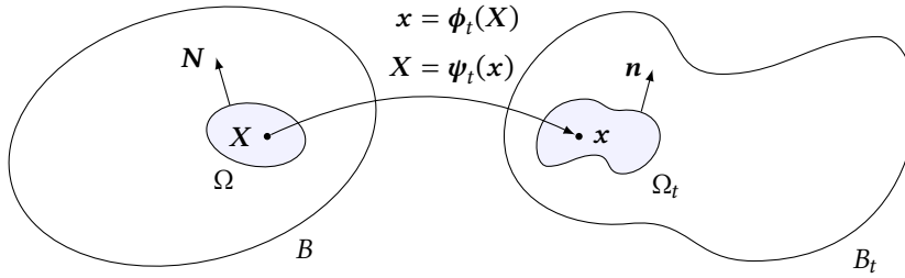
Figure 7.3: The deformation \phi_t(X) maps the body B \subset \mathcal{E}_3 to B_t \subset \mathcal{E}_3 at time t . The inverse of \phi_t at time t is \psi_t . An arbitrary part \Omega of B is mapped to \Omega_t .
