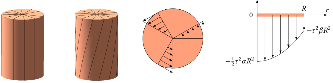
Figure 14.2: From the left: The first two figures depict the cylinder before and after twisting. The third and fourth figures show the horizontal and vertical components of the traction applied to the cylinder's top.
