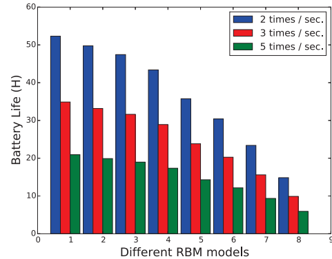
Fig. 3: Smartwatch battery Life under various sizes of RBM models within the activity recognition pipeline. Model IDs (x-axis) shown correspond to those listed in Table IV. For each model, the impact of three batch periods are shown. Model ID 3 matches the default RBM architecture evaluated in Section III.
