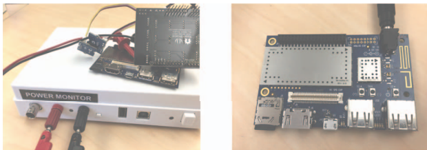
Fig. 2: Experimental setup, including: Snapdragon 400 development board, power monitor and additional sensors as required.
