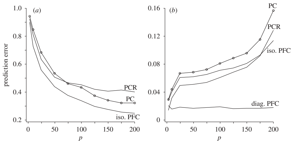
Figure 3. Comparison of prediction errors from PCR (equation (2.2)), inverse PCs (equation (4.2)), isotonic principal fitted components (iso. PFC) (equation (4.4)) and diagonal principal fitted components (diag. PFC) (equation (4.5)): (a) isotonic PFC, \mathbf{f}_y = (y, y^2, y^3)^T ; (b) diagonal PFC, f_y = y .
