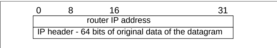
Figure 3-32 ICMP: Redirect
