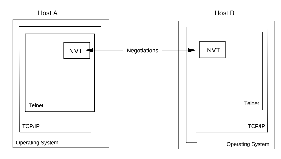
Figure 13-2 Telnet negotiations
