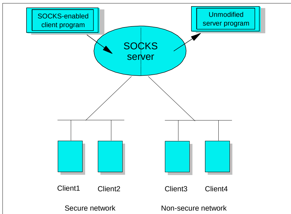
Figure 22-18 Circuit-level gateway
