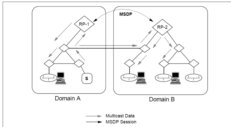
Figure 6-14 MSDP operations
