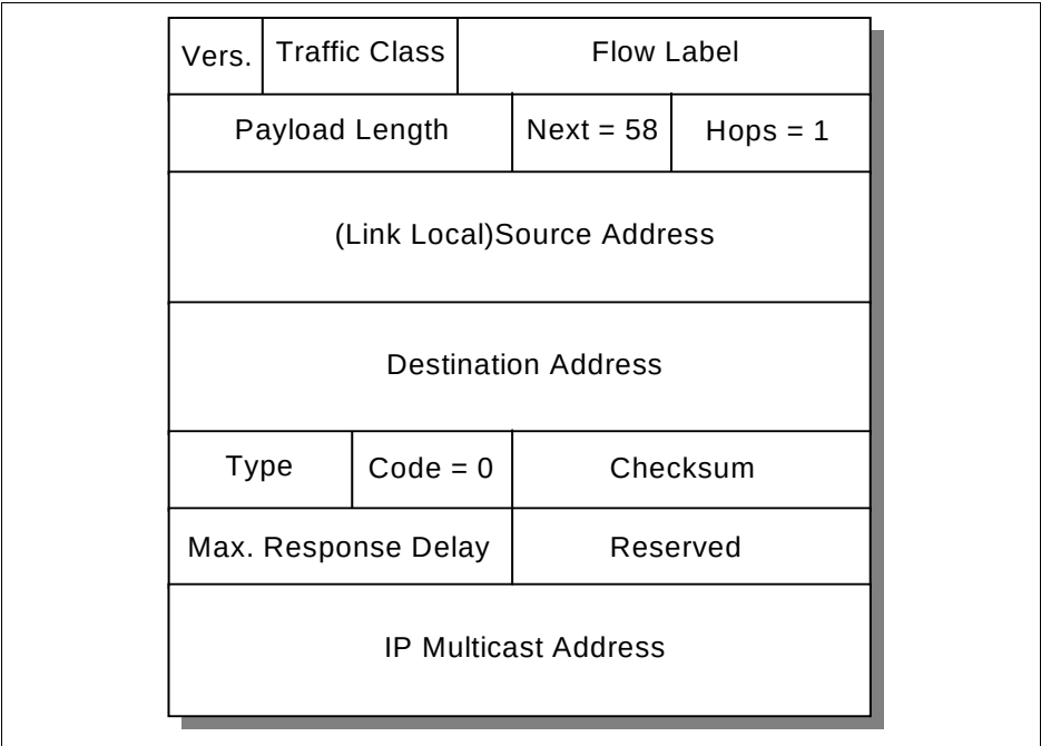
Figure 9-22 MLD message format
