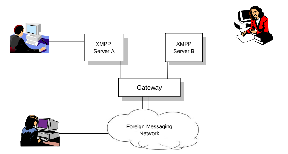
Figure 19-7 XMPP architecture
