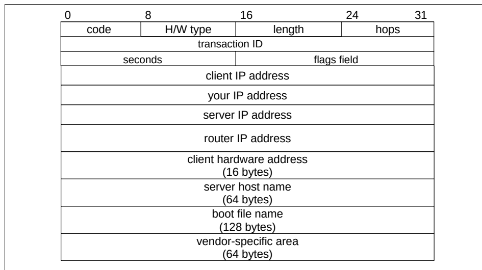
Figure 3-43 BOOTP message format
