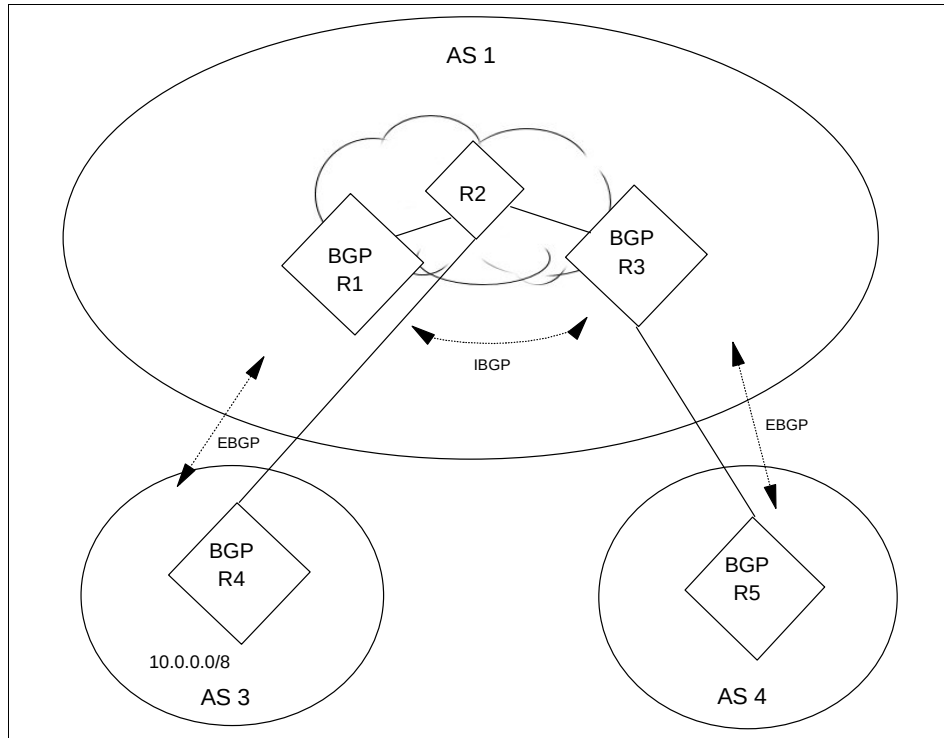
Figure 5-26 BGP synchronization
