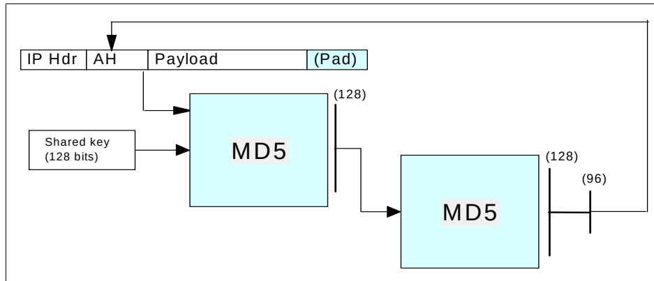
Figure 22-8 HMAC-MD5-96 processing
