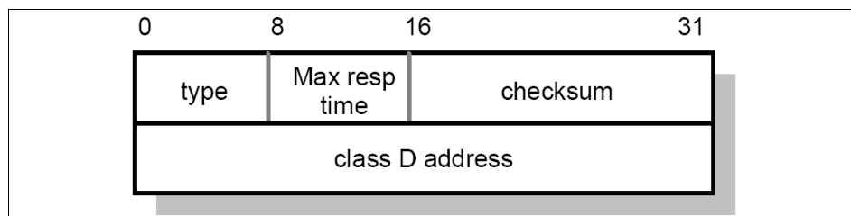
Figure 6-2 IGMP message format
