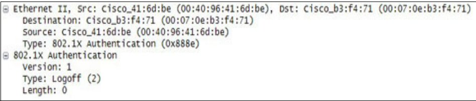
Figure 23-21 EAPoL-Logoff packet
