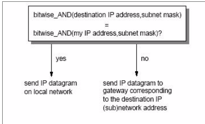
Figure 3-8 IP: Routing with subnets
