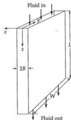
2B.3 Laminar flow in a narrow slit (see Fig. 2B.3).
