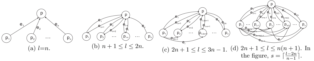
Figure 1: Achieving the maximum PageRank scores.
