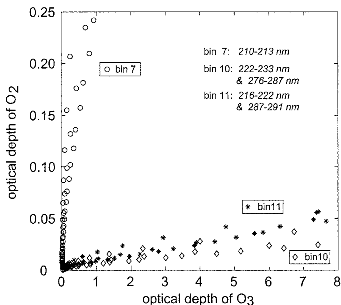
Figure 7. Slant-column optical depths in O 2 and O 3 to the sun, sampled from the different stratospheric altitudes (16–80 km) and different SZA 0°–80° for a January tropical atmosphere. Results are shown for the three super-wide bins of Fast-J2 (nos. 7, 10, and 11) that include both O 2 and O 3 absorption. The tight correlation for each bin demonstrates that the relative amounts of attenuation by these two absorbers remains nearly constant over a wide range of conditions.
