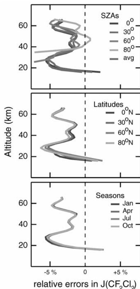
Figure 6. The relative error in J(\text{CF}_2\text{Cl}_2) (%) as a function of altitude calculated with Fast-J2 (compared with UCI standard model). Results are shown for (a) a range of solar zenith angles (SZA) and their 24-hour average with the U.S. Standard Atmosphere, (b) a range of latitudes in April (USAF reference atmospheres) with overhead sun, and (c) a range of seasons at 30^\circ\text{N} with overhead sun. The latter two cases show only the sensitivity to changes in the background atmosphere.
