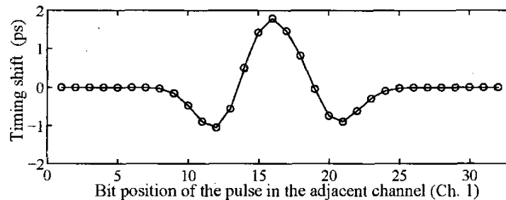
Figure 1. Timing shift G_{1i} of the target pulse in the center channel (Ch. 2) induced by interaction with a pulse in bit position i in one of the adjacent channels (Ch. 1). The target pulse is at bit 16. The propagation distance of the WDM RZ system is 5000 km, the amplifier spacing 50 km, the channel spacing 35GHz and bit rate 10GB/s.
