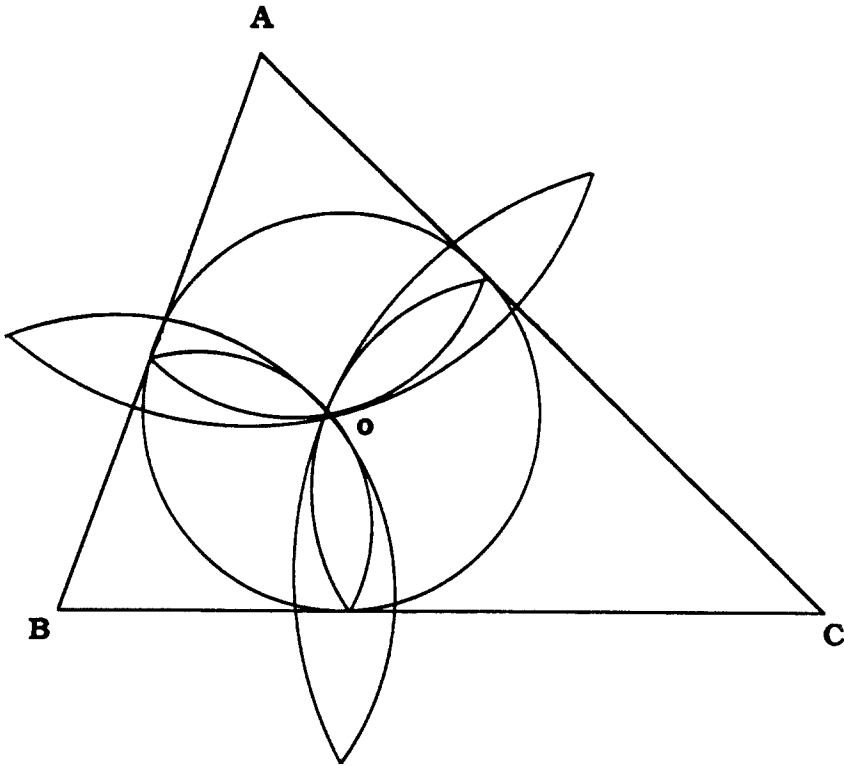
Figure 1. The petals of the win-set and half-win set around o , the center of the yolk
