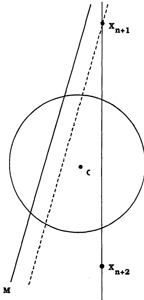
Figure 4. Construction used in proof of Theorem 4
