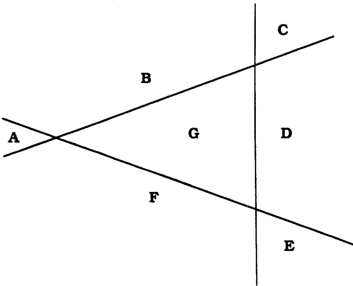
Figure 3. Construction used to prove Theorem 3
