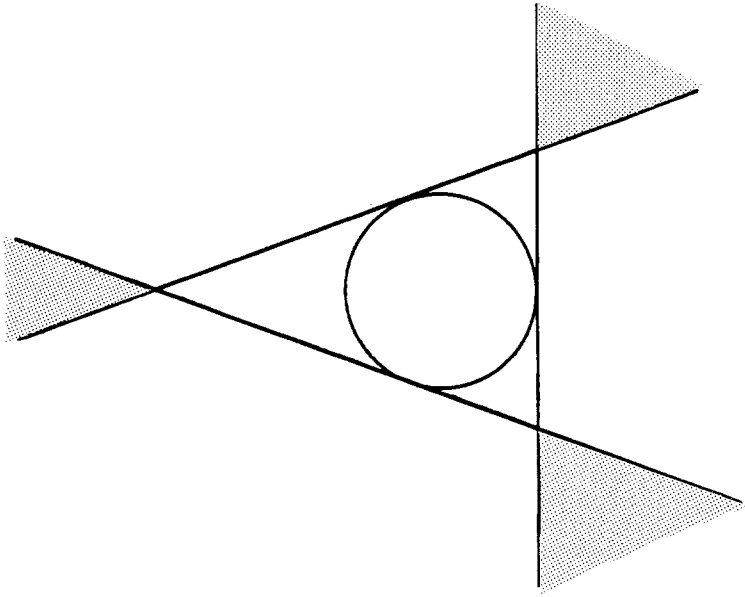
Figure 2. Median triangle bounding the yolk
